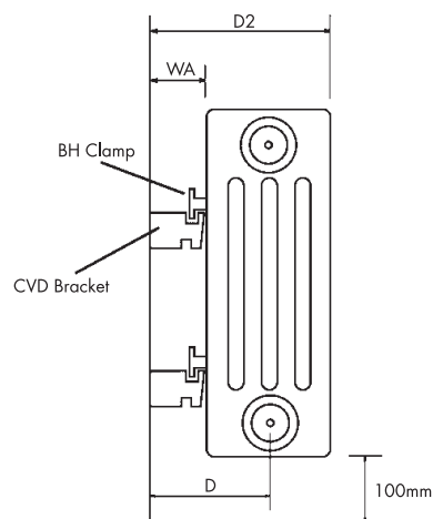
Measurements using 10mm CVD Bracket Slot (add 5mm if using 15mm Slot)
