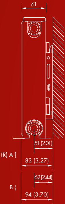
Side View - Horizontal Panel
